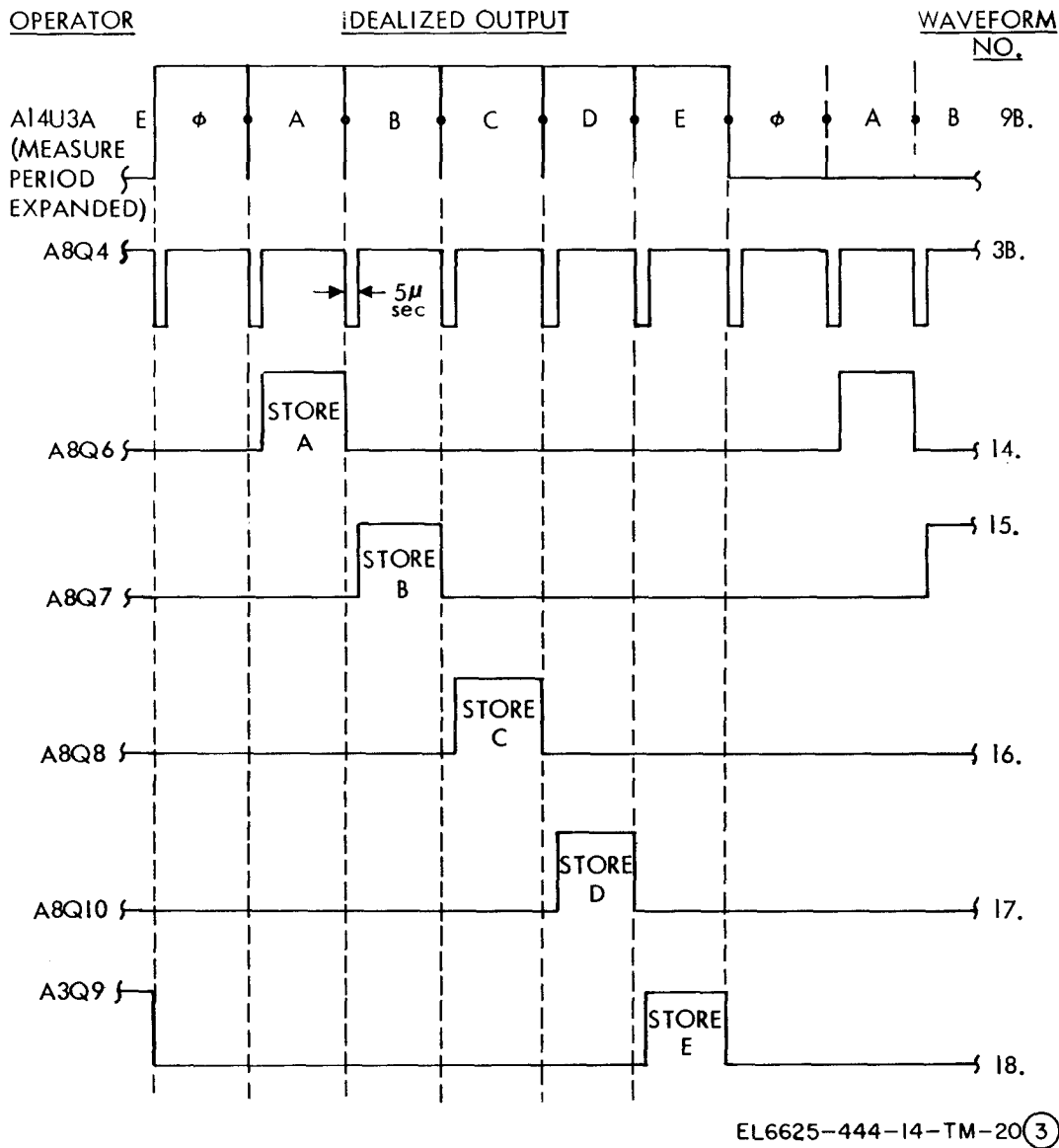
Figure 5-5 (3) Timing and synchrony diagram (sheet 3 of 3).
