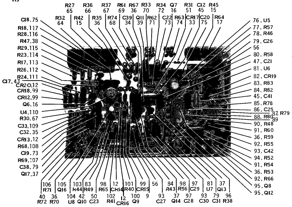
B-15. Ac converter assembly
