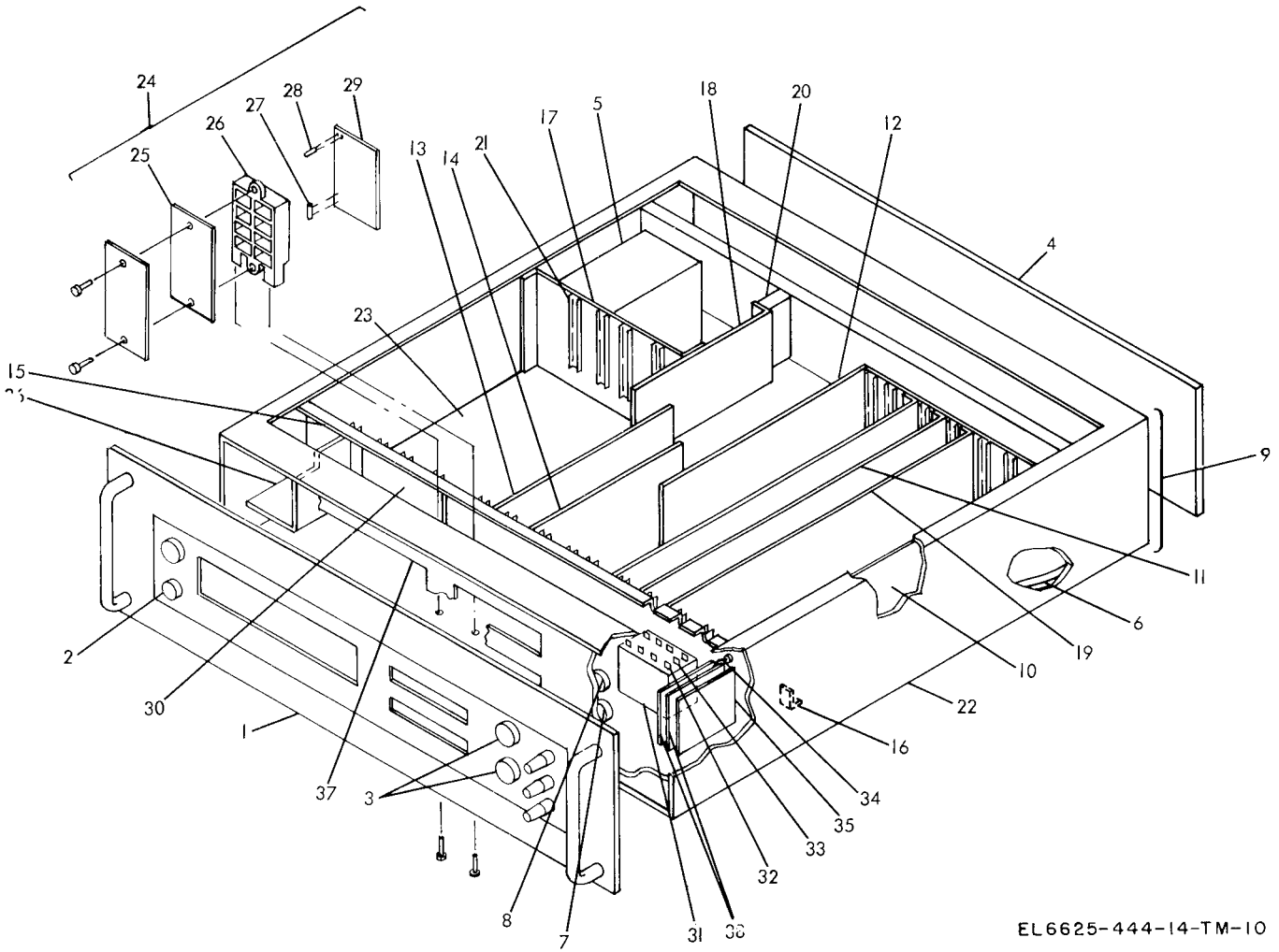
Figure 10. Chassis assembly
