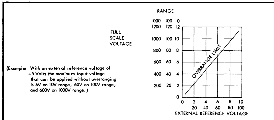
Figure 3-4. Ratio overrange limits.
