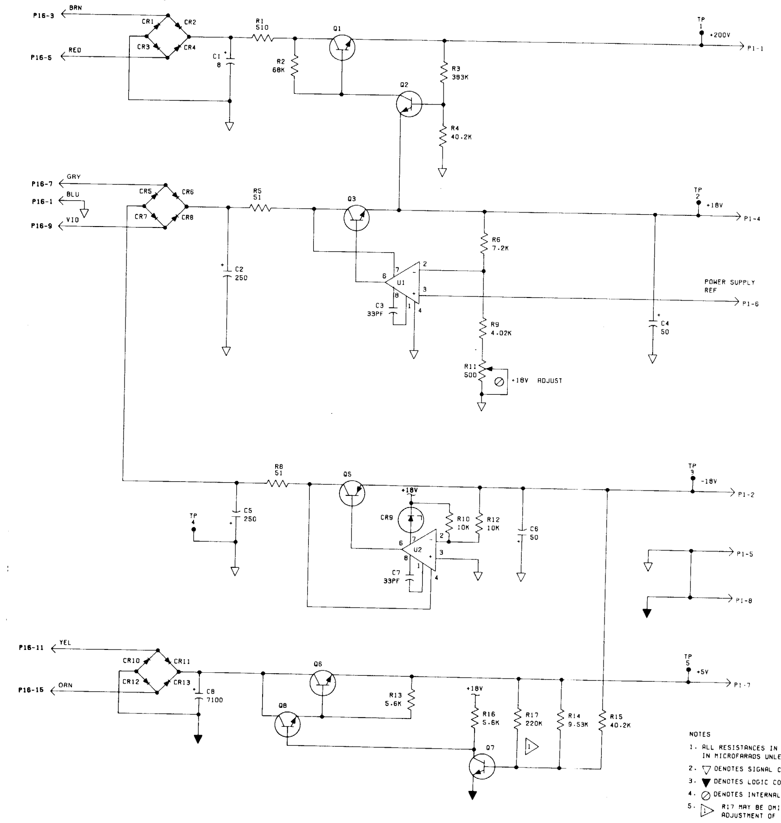
Figure FO-8. Power supply (A1) schematic diagram.
