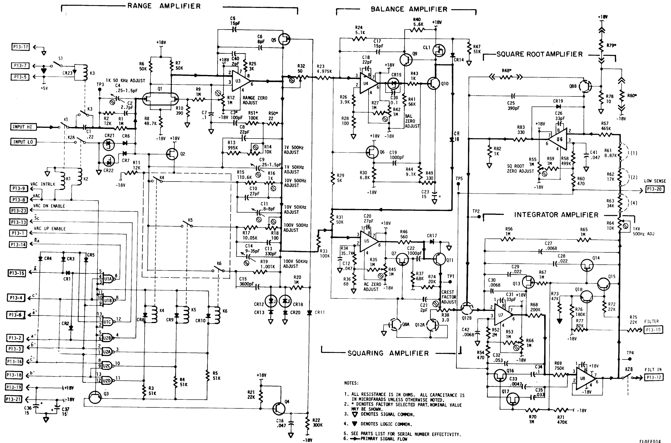
Figure FO-12. Ac converter, schematic diagram.
