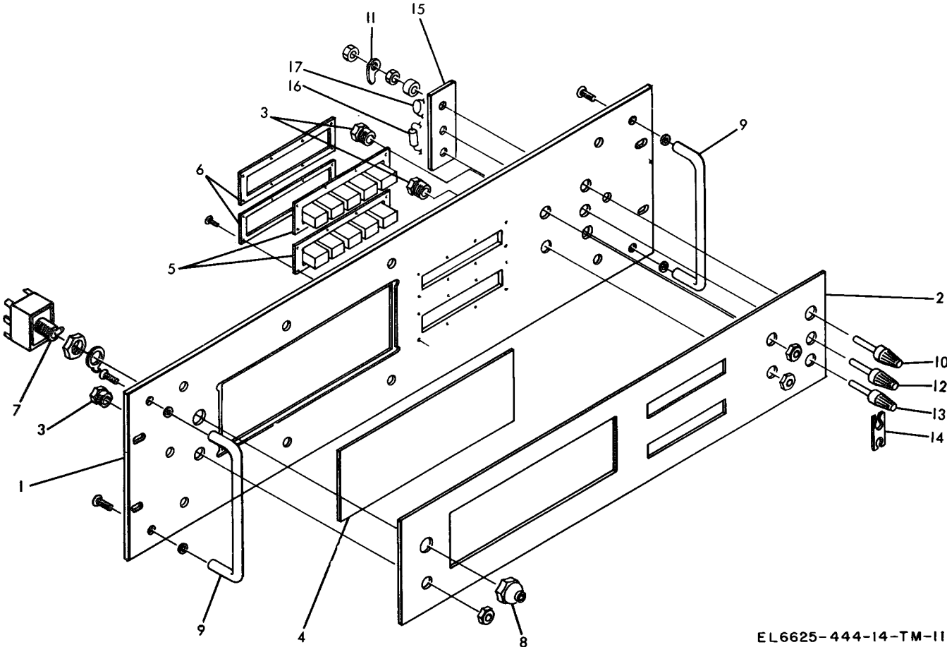
Figure 11. Front panel assembly.
