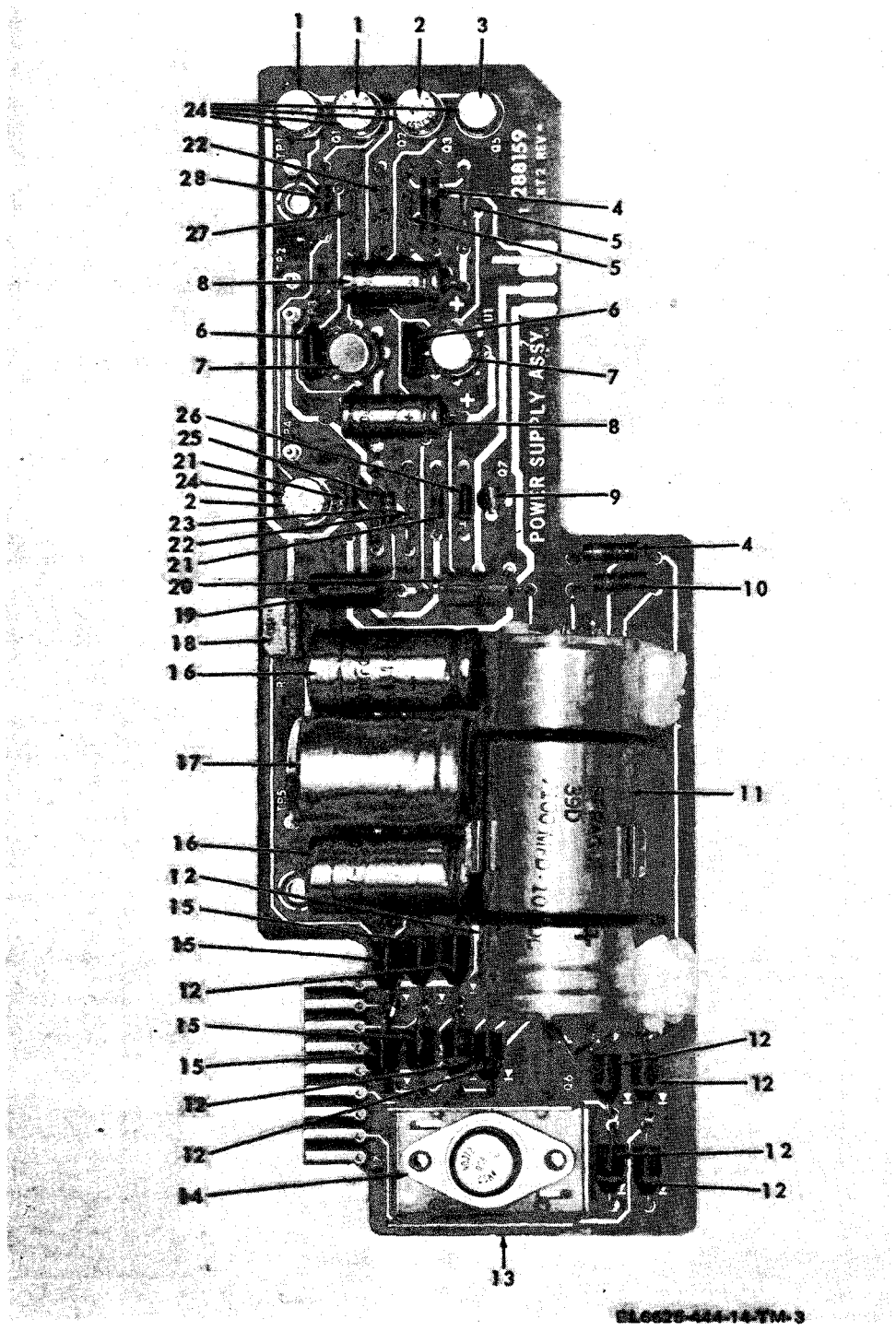
Figure 3. Power assembly.
