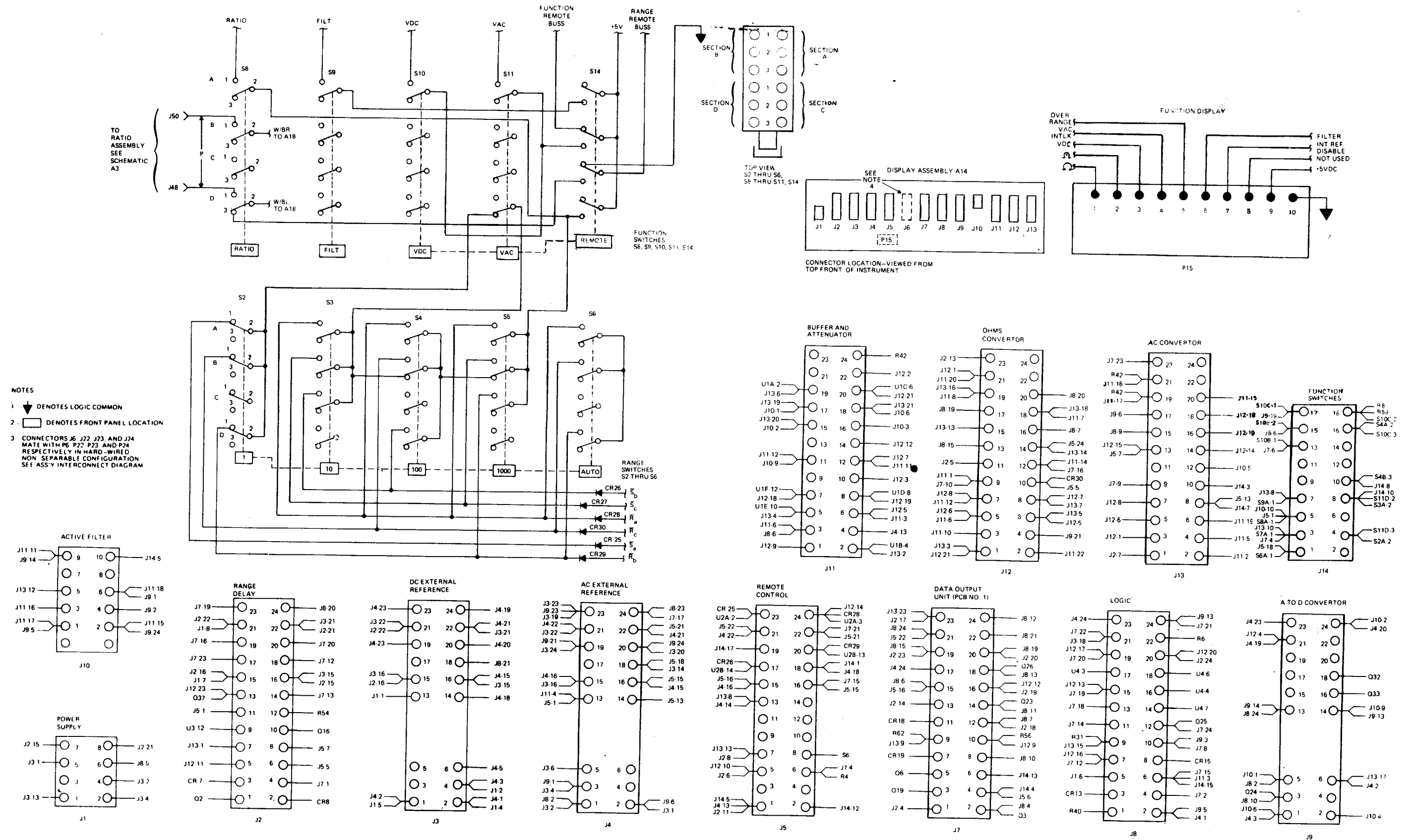
Figure FO-6 ( ) . Display (A14) schematic diagram (sheet 1 of 2).
